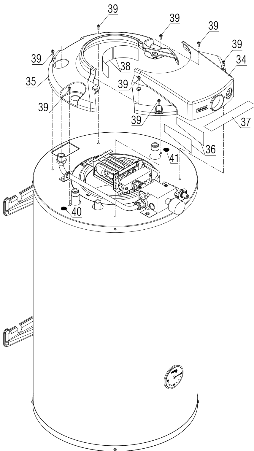
View G
